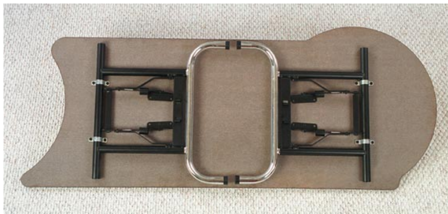
Underside of desk shown in folded position
